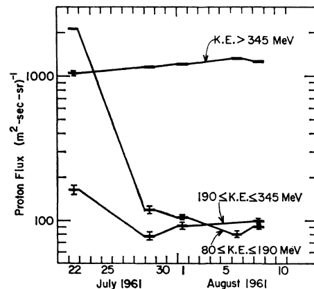
FIG. 5. The primary proton flux at 0 \text{ g/cm}^2 as a function of time for three energy intervals during July and August 1961.
